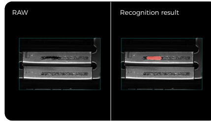
Defect detection
