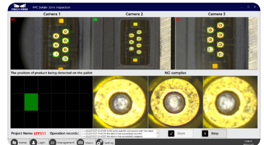
Software Interface
