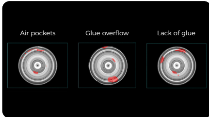
Defect classification
